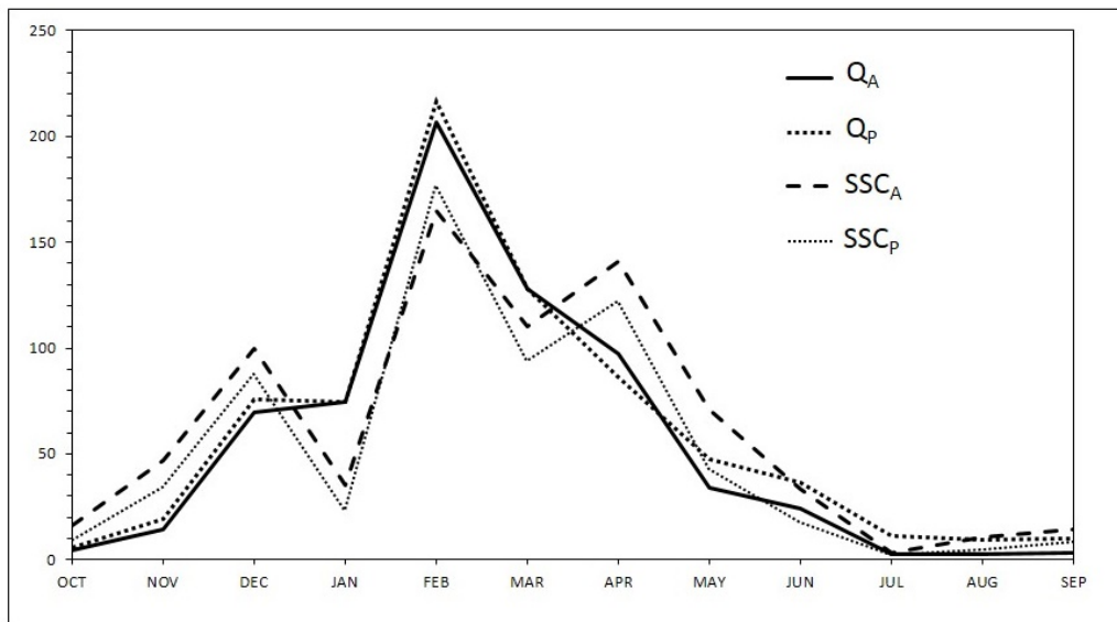
Figure 5. Monthly variations of water flow ( \text{m}^3/\text{s} ) and SSC ( \text{mg}/\text{L} ) [Q: flow; (A): Agia Paraskevi and (P): Palaioopyrgos]
